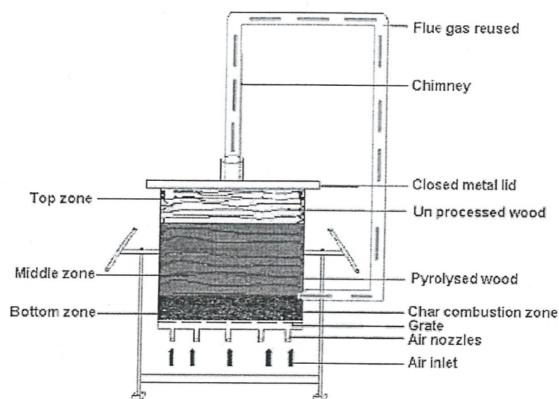
Figure: Retort Type Kilns
